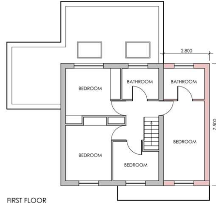
FIRST FLOOR PROPOSED
