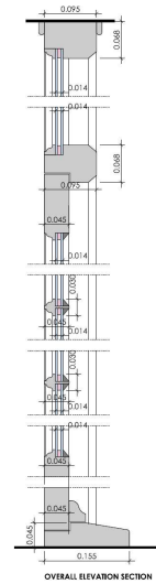
FRENCH DOORS 01 PAINTED HARDWOOD SLIMLINE HERITAGE DG FRENCH DOORS
