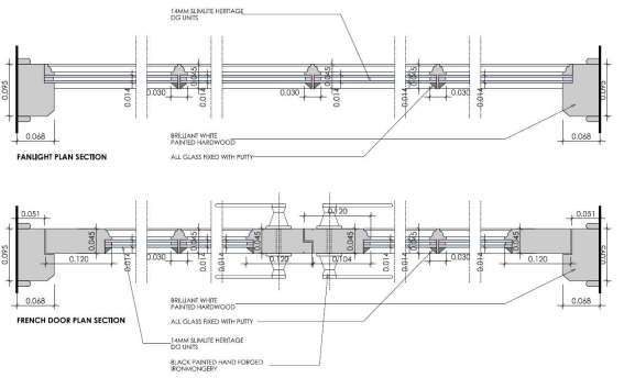
FRENCH DOORS 01 PAINTED HARDWOOD SLIMLINE HERITAGE DG FRENCH DOORS
