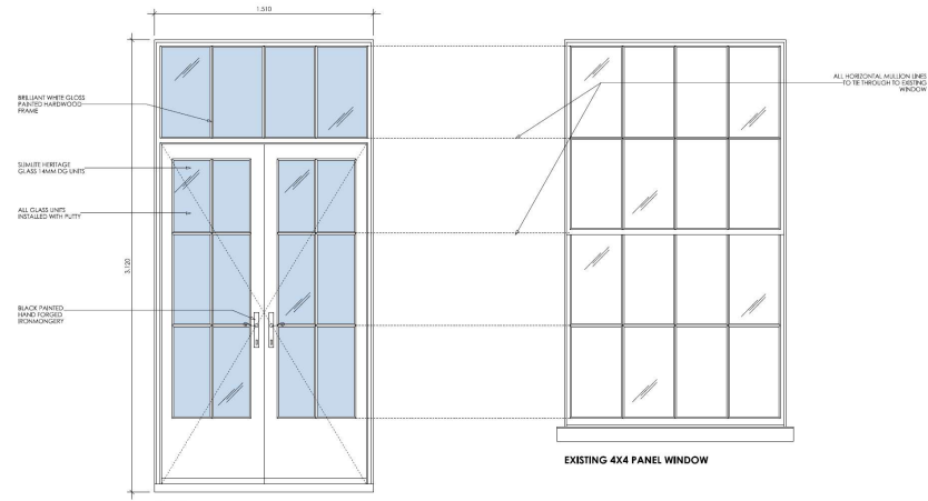
FRENCH DOORS 01 PAINTED HARDWOOD SLIMLINE HERITAGE DG FRENCH DOORS SEE DRAWING NO. A-701 FOR 1:2 SCALE PROFILE DETAILS
