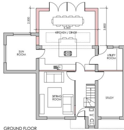
GROUND FLOOR PROPOSED
