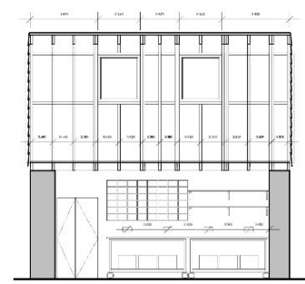
Long Section 1:50@A3
