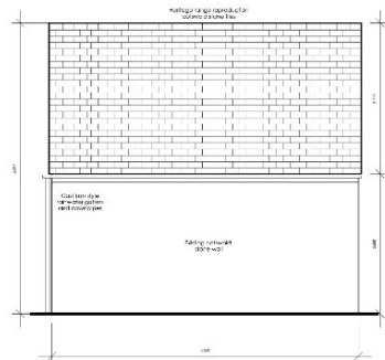
East Elevation 1:50@A3
