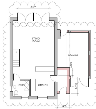
GROUND FLOOR PROPOSED
