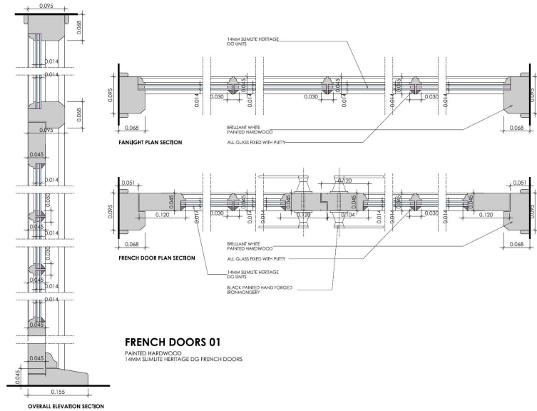
FRENCH DOORS 01 PAINTED HARDWOOD SLIMEST HERITAGE DG FRENCH DOORS SEE DRAWING NO. A-701 FOR 1:2 SCALE PROFILE DETAILS
