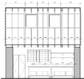
Long Section 1:50@A3
