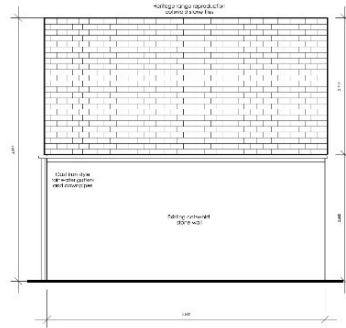
East Elevation 1:50@A3
