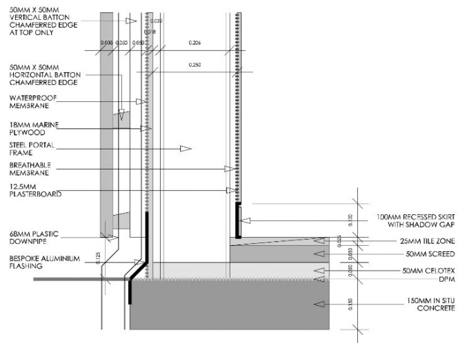
DETAIL 1
