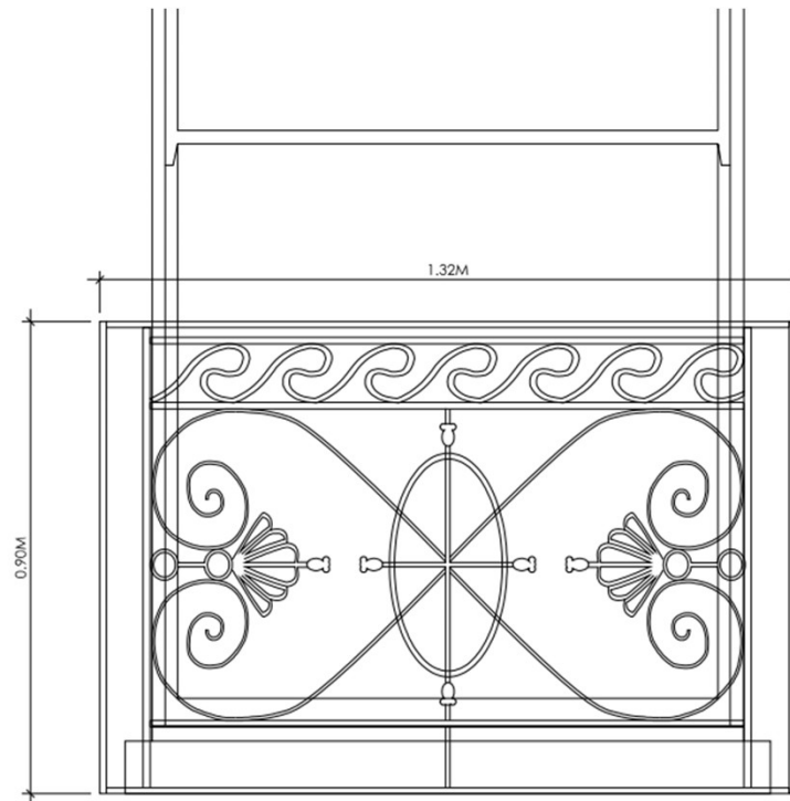
ENLARGED DETAIL PROPOSED
