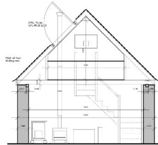
Short Section 1:50@A3
