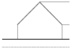
REAR ELEVATION PROPOSED
