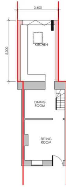
GROUND FLOOR PROPOSED
