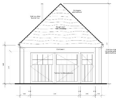
South Elevation 1:50@A3
