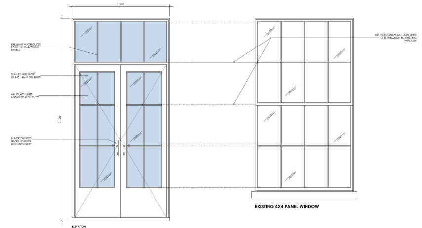
FRENCH DOORS 01 PAINTED HARDWOOD SLIMEST HERITAGE DG FRENCH DOORS SEE DRAWING NO. A-701 FOR 1:2 SCALE PROFILE DETAILS
