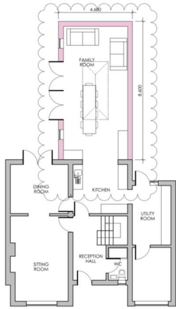
GROUND FLOOR PROPOSED
