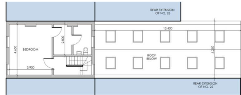
FIRST FLOOR PROPOSED
