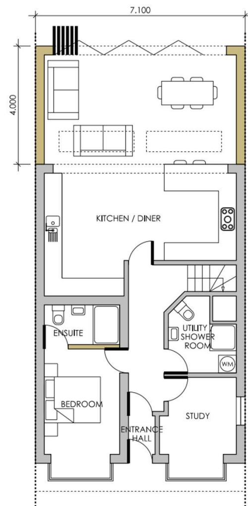
GROUND FLOOR PROPOSED
