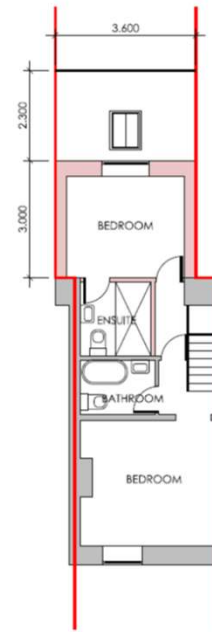
FIRST FLOOR PROPOSED
