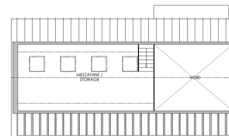
FIRST FLOOR PROPOSED
