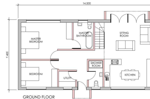
GROUND FLOOR PROPOSED
