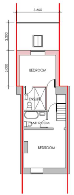
FIRST FLOOR PROPOSED
