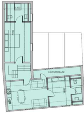
SECOND FLOOR PROPOSED
