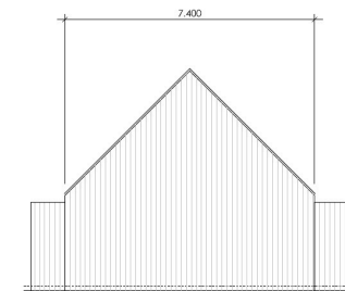
SIDE ELEVATION PROPOSED
