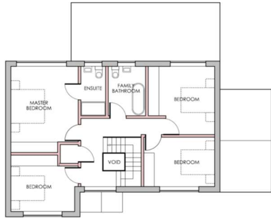
FIRST FLOOR PROPOSED
