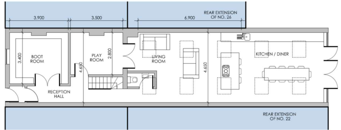
GROUND FLOOR PROPOSED
