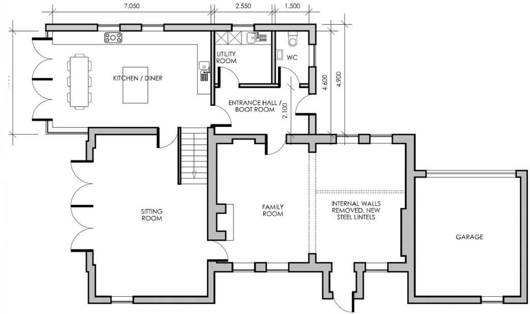
GROUND FLOOR PROPOSED
