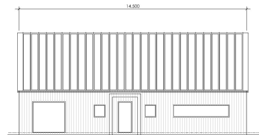
FRONT ELEVATION PROPOSED
